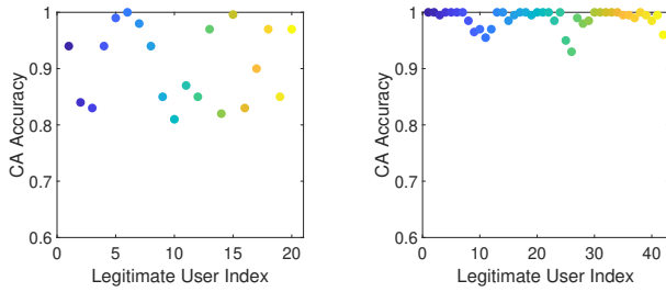
Fig. 10. CA accuracy of TrueHeart using the PPG measurements from the wrist areas and the fingertips.
