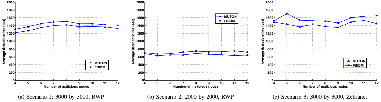
Fig. 4. Detection time versus number of malicious nodes under three different scenarios.
