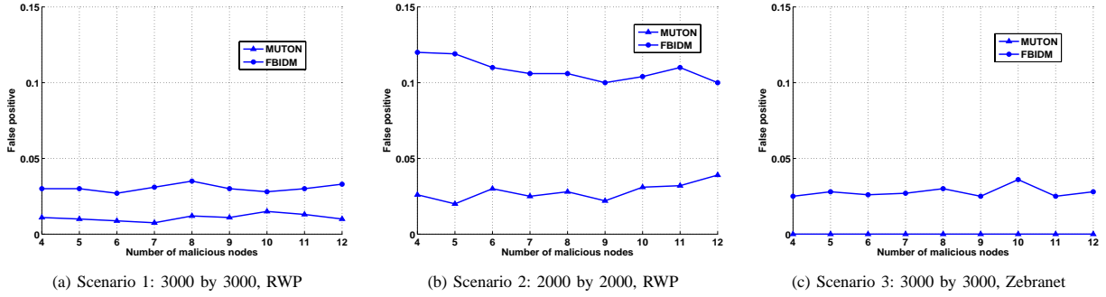
Fig. 5. False positive rate versus number of malicious nodes under three different scenarios.
