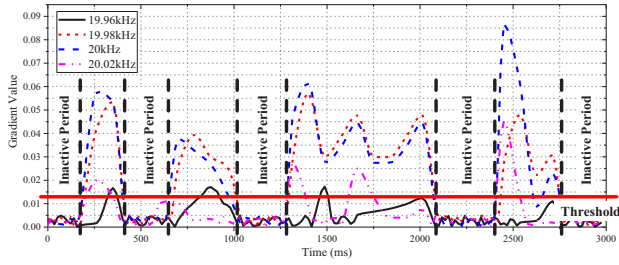
Fig. 5. Doppler profiles of lip movements when a user speaks four words under four frequencies.
