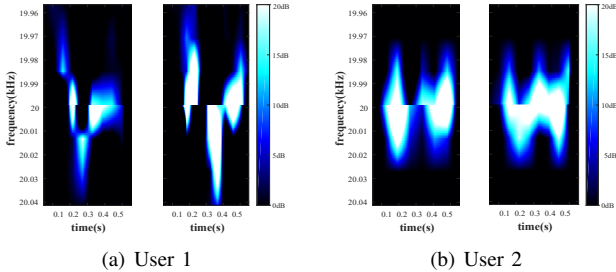
Fig. 3. Doppler profiles of acoustic signals caused by speaking the word ‘World’ under two different users.
