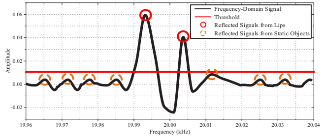
Fig. 10. An example of the reflected signals from speaking lips and static objects.
