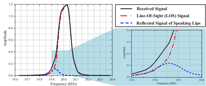
Fig. 1. An example of a mixed received signal including a LOS signal and a reflected signal from speaking lips.
