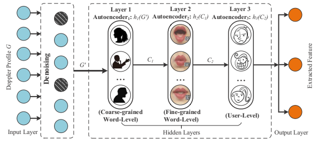
Fig. 6. Architecture of feature extraction through a three-layer autoencoder-based Deep Neural Network.
