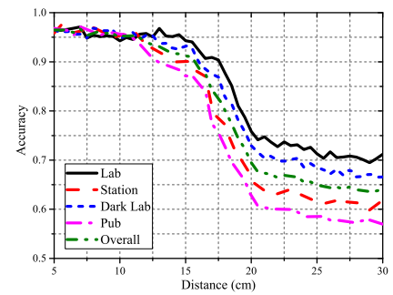
Fig. 16. Relationship between authentication accuracy and distances from microphone to users' lips in four different environments.
