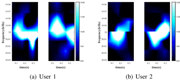
Fig. 2. Doppler profiles of acoustic signals caused by speaking the word ‘Hello’ under two different users.
