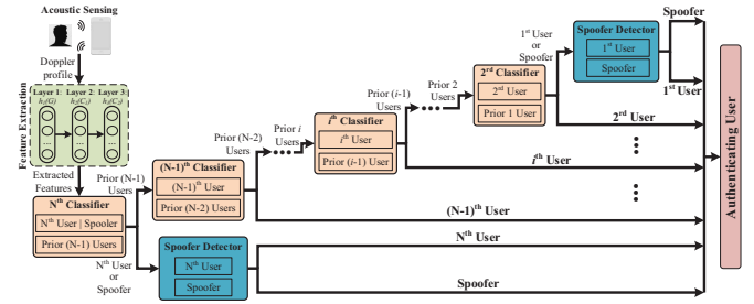
Fig. 8. Architecture of the binary tree-based authentication under single word.
