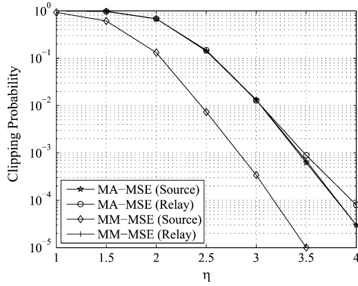
Fig. 9. Example 5: Clipping probability versus \eta . N_s = N_r = N_d = 3 , N_b^{[n]} = 2 , \text{SNR}_s = \text{SNR}_r = 20 dB.
