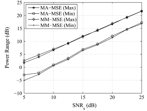
Fig. 7. Example 5: Power range versus \text{SNR}_s . N_s = N_r = N_d = 3 , N_b^{[n]} = 2 , \text{SNR}_r = 20 dB.
