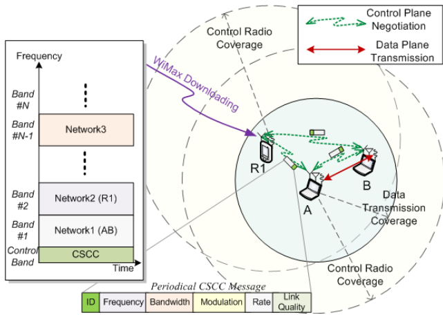
Figure 2. The CSCC spectrum coordination protocol.
