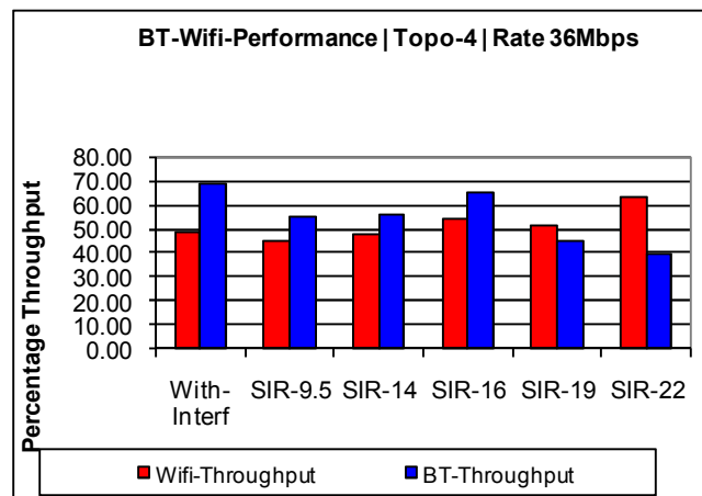
Figure 11. SIR-BT scheme with Fixed link Rate at 36Mbps for multiple SIR budget threshold values.
