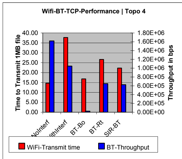
Figure 10. WiFi-g-1Mbyte TCP file transfer time and BT throughput in Topology 4.
