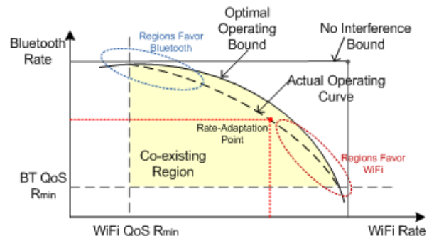
Figure 2. Coexistence Region of Operation for BT-Wifi.
