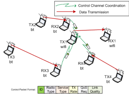
Figure 3. CSCC protocol in an IEEE 802.11g and Bluetooth coexistence scenario.
