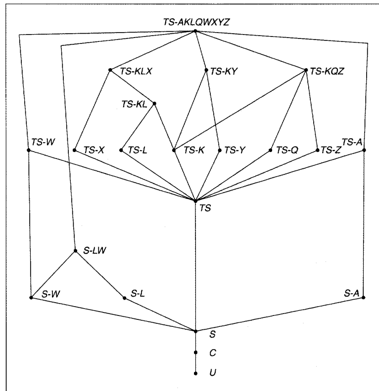
Figure 3. Smith's lattice.
