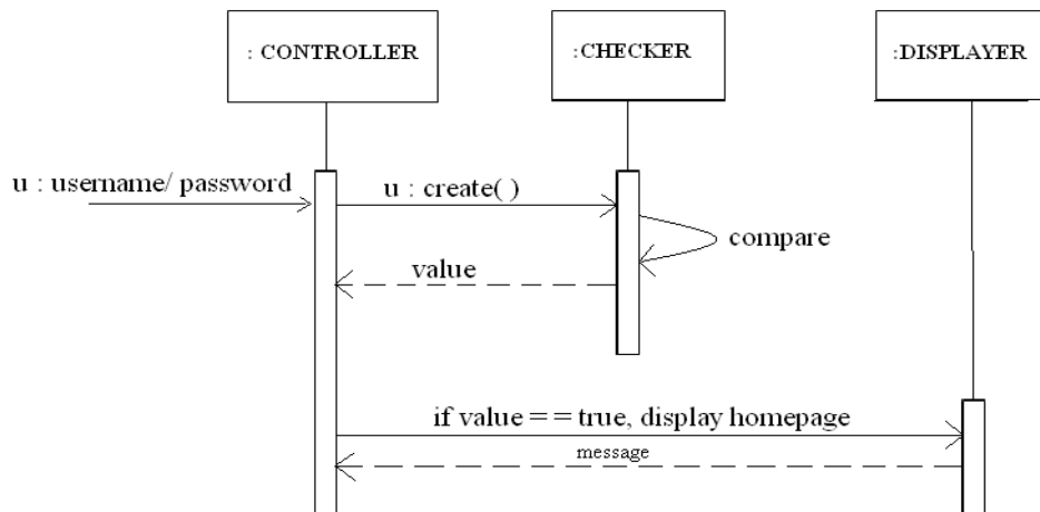
Fig 4: Use Case #2 and #3 Interaction Diagram
