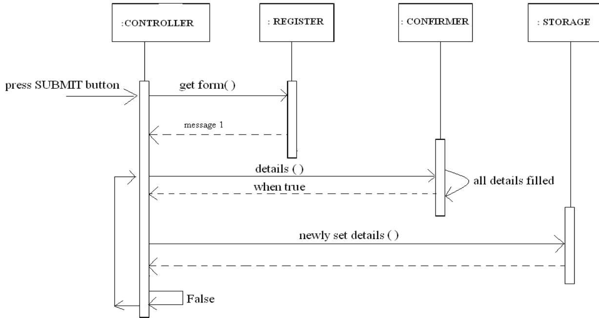
Use Case #2 ( Create Account)
