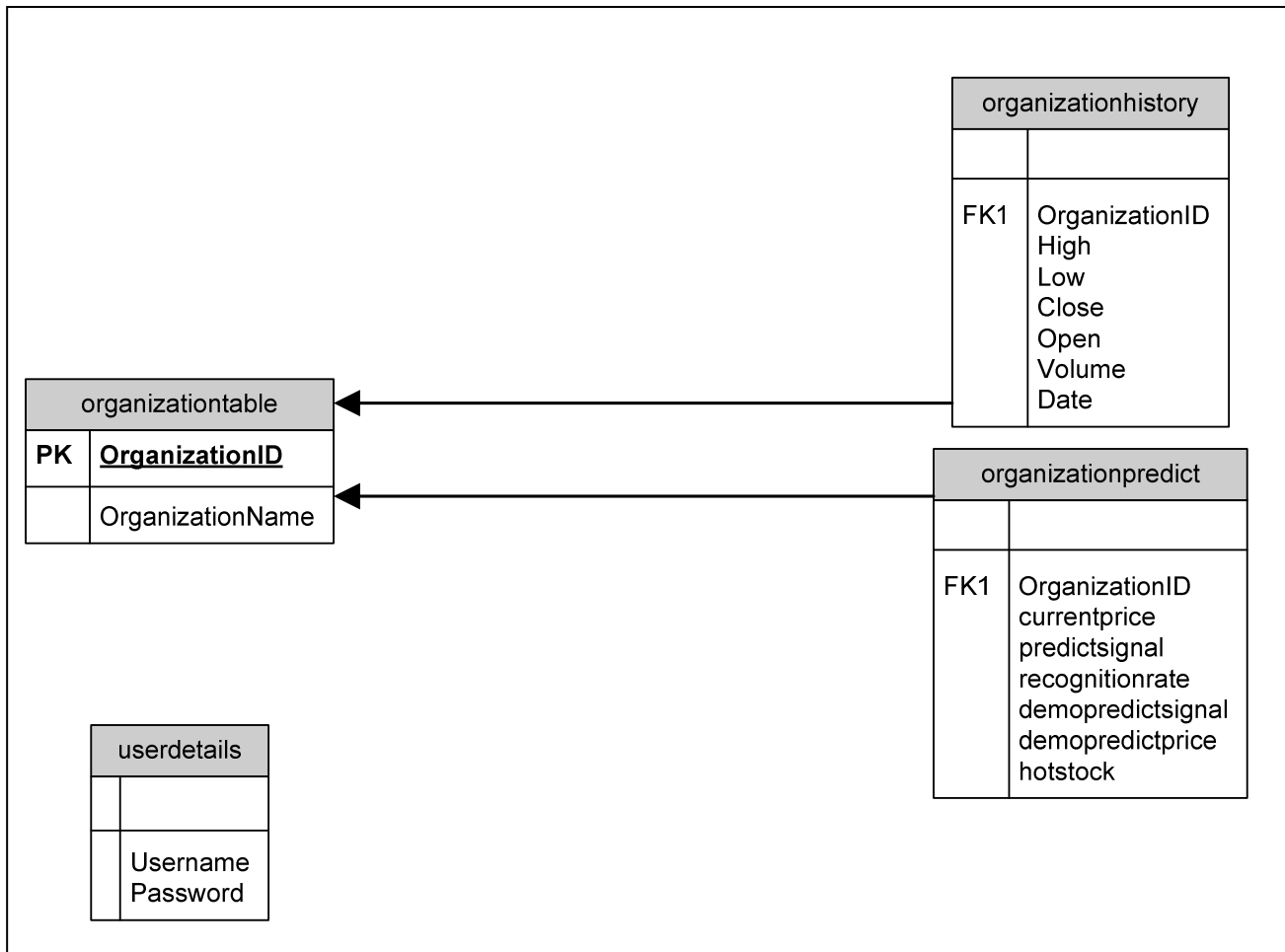
Fig 14: Database Schema
