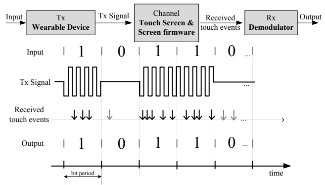
Fig. 3. Capacitive touch screen communication showing OOK modulation and variations in number and timing of generated events
