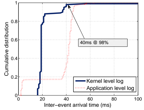
Fig. 11. CDF of inter-event arrival times of events captured at application level and kernel level log files with 10 Volt peak-to-peak 1KHz square wave input signal
