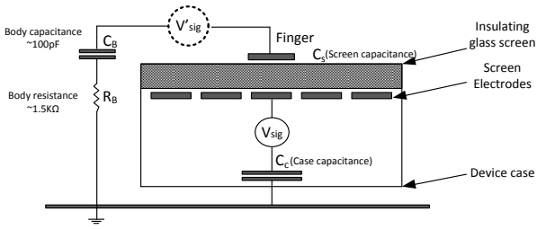
Fig. 1. Schematic of a basic capacitive touchscreen
