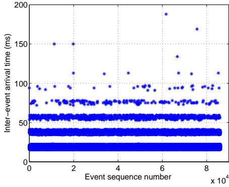
Fig. 10. Distribution of inter-event arrival times of events generated by a 10 Volt peak-to-peak 1KHz square wave signal captured in kernel level log files
