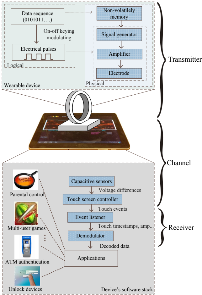
Fig. 5. Overall architecture of the capacitive touch communication system
