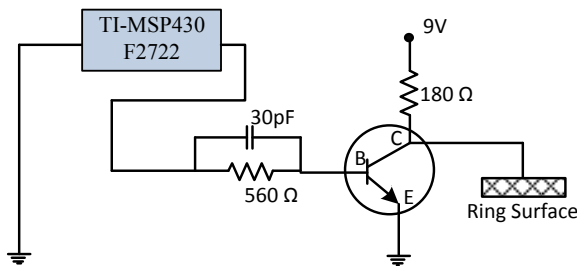
Fig. 15. Schematic of the custom-built ring
