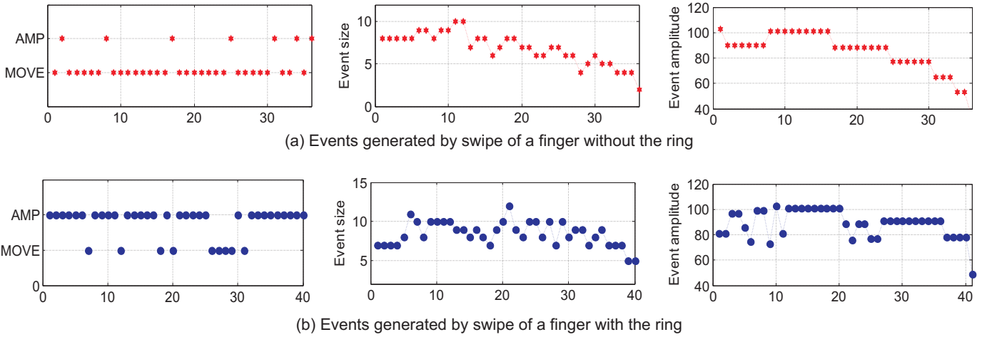
Fig. 8. Type, Size and Amplitude values generated from finger swipes with and without the ring. A ring bearing finger produces many AMP events while swipe without ring induces correlation between Size and Amplitude
