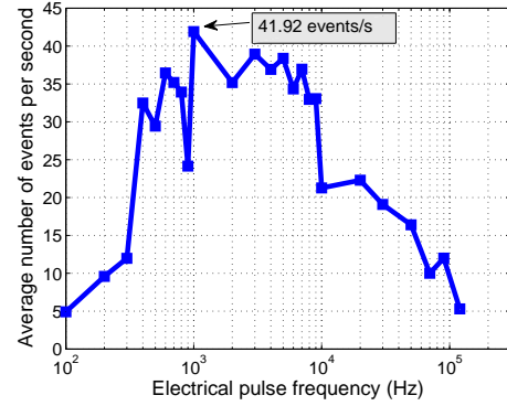
Fig. 9. Touchscreen responses to 10 Volt peak-to-peak square wave signals with different frequencies ranging from 100Hz to 120KHz (log scale)
