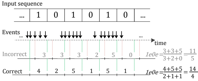
Fig. 6. Offline calibration process searching for the correct bit synchronization point at which the 1e0e ratio reaches the maximum value
