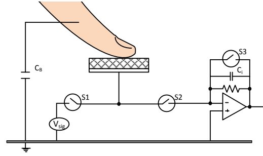
Fig. 2. Internal touch detection circuit
