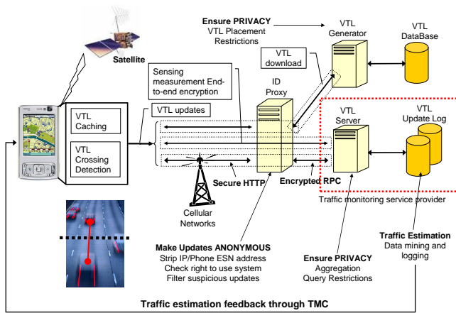
Figure 2: Virtual Trip Line: Privacy-Preserving Traffic monitoring System Architecture.
