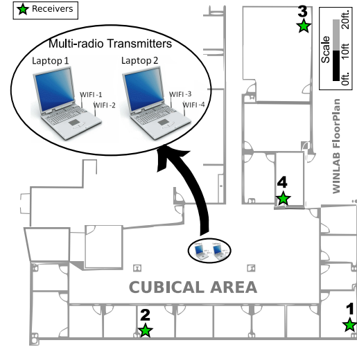
Figure 2. Floorplan of the experiment environment and the node placement
