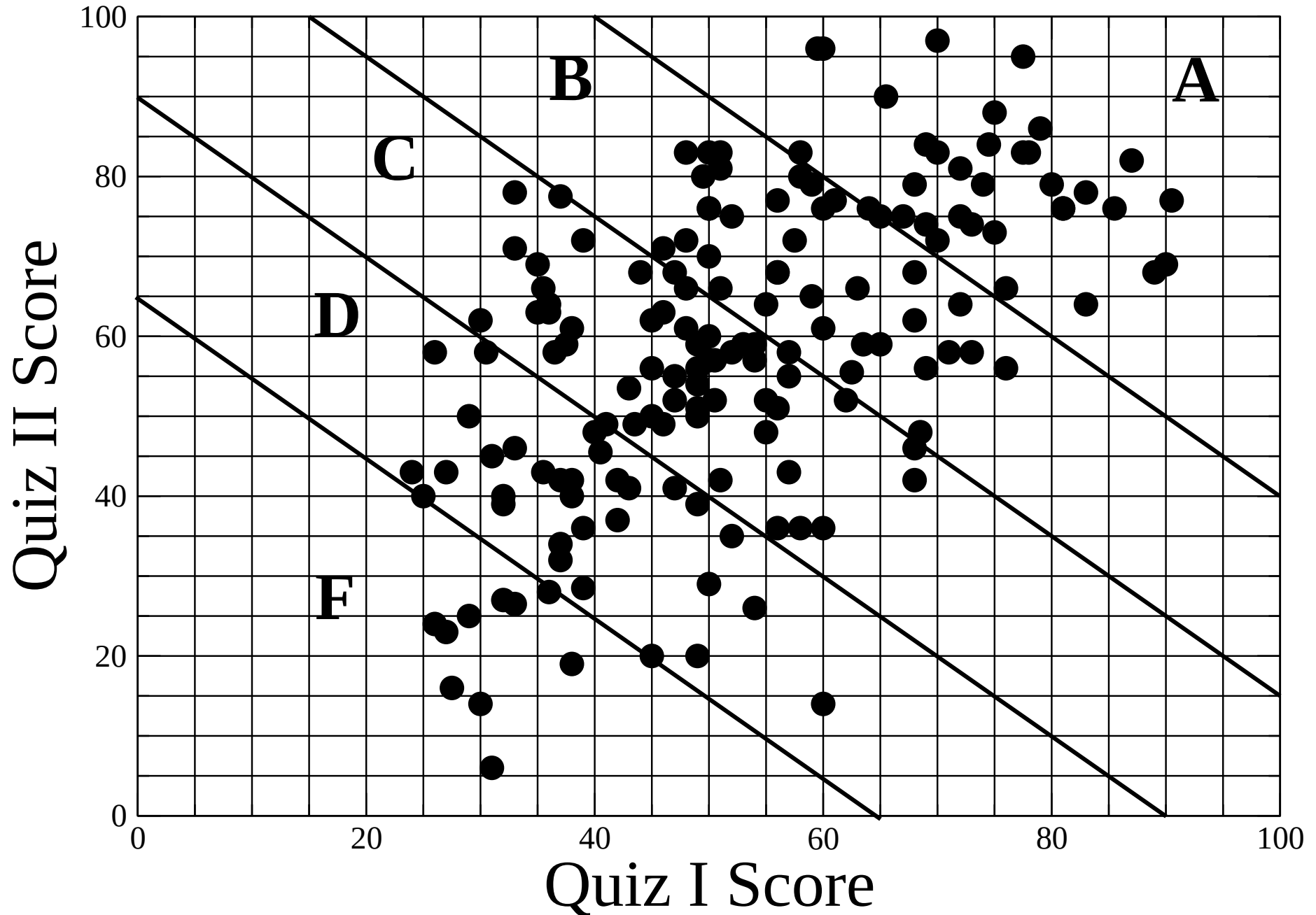
Scatterplot
